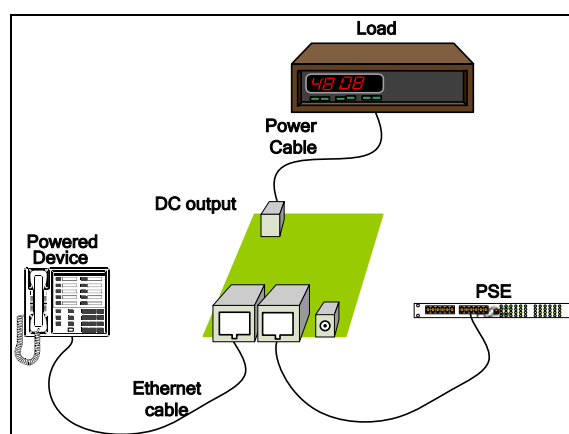
Figure 9: Test Setup
