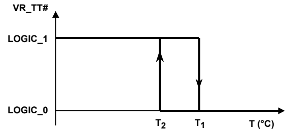
FIGURE 39. TEMPERATURE HYSTERESIS OF VR_TT#
