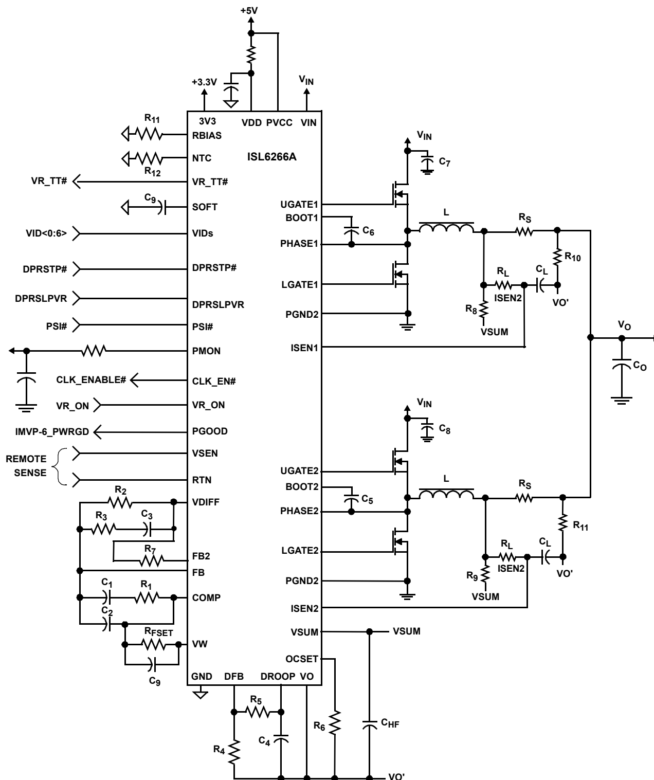
FIGURE 33. ISL6266A BASED TWO-PHASE BUCK CONVERTER WITH RESISTIVE CURRENT SENSING
