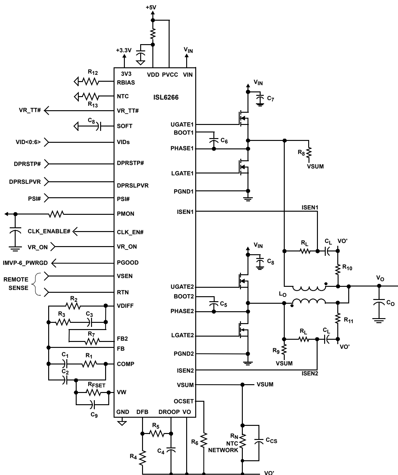
FIGURE 31. ISL6266 BASED TWO-PHASE COUPLED INDUCTOR DESIGN WITH DCR SENSING
