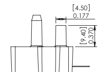
F- Port A Cut 0.370" Configuration
