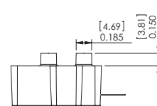
D- Two Ports Cut 0.150" Configuration
