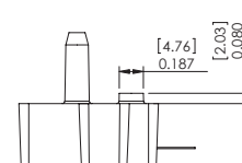
E- Port A cut 0.080" Configuration
