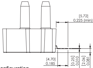
J- Jogged Bend Configuration
