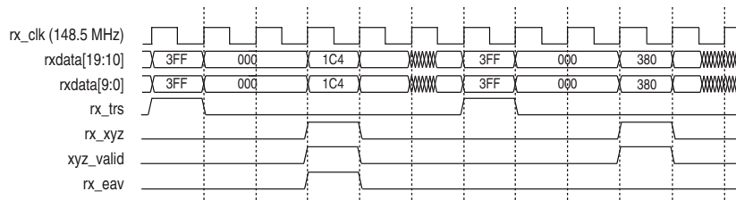
Figure 3-36. Behavior of rx_trsr, rx_xyz, xyz_valid and rx_eavr Signals—425MA
