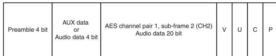
Figure 4-5. AES Format
