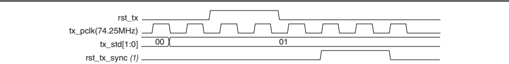
Figure 3-30. Power-up Reset for the Transmitter
