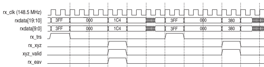
Figure 3-37. Behavior of rx_trsr, rx_xyz, xyz_valid and rx_eavr Signals—425MB
