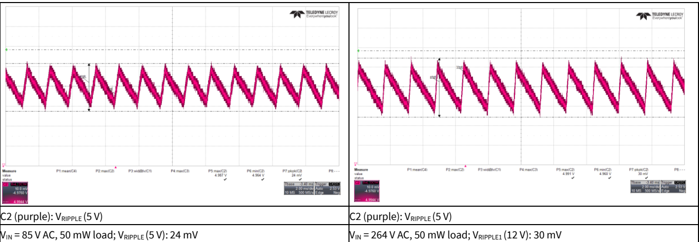
Figure 21 Output ripple voltage in ABM 50 mW load
