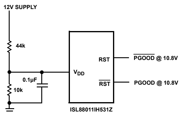
FIGURE 13. 12V SUPPLY PGOOD or \overline{PGOOD}
