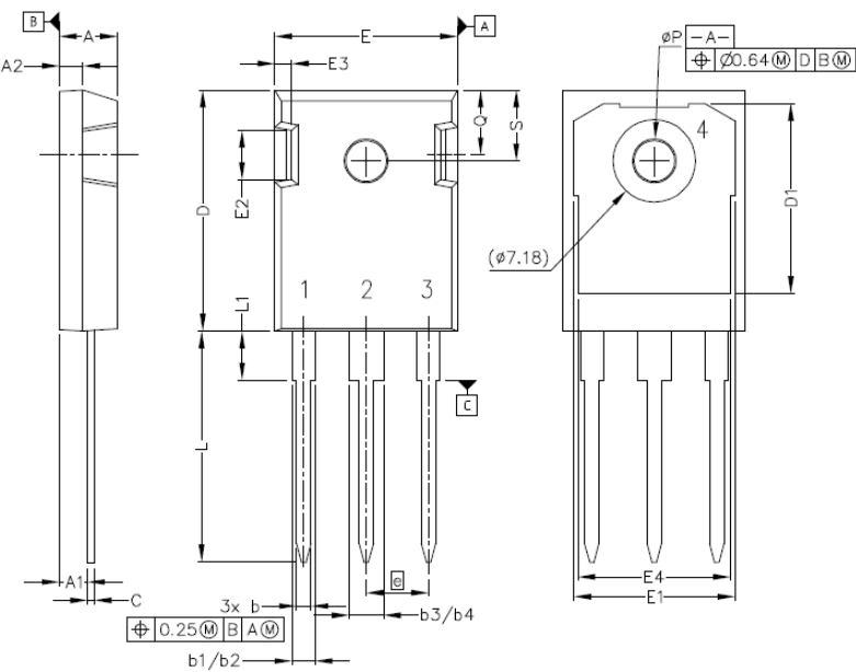
Package TO-247-3
