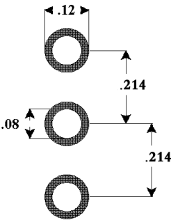
TO-247-3
