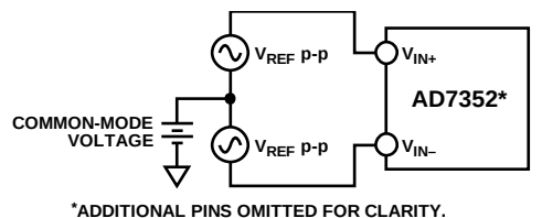
Figure 19. Differential Input Definition
