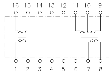
Schematic C
