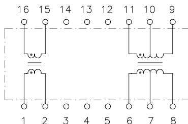
Schematic B
