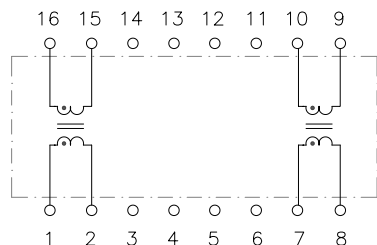
Schematic A
