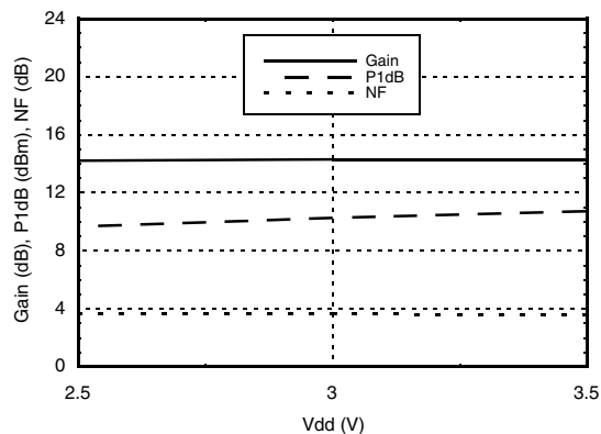
Gain, Noise Figure & Power vs. Supply Voltage @ 24 GHz
