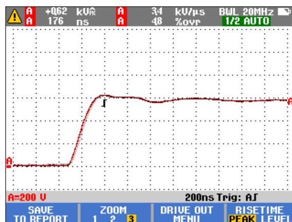
Voltage modulation with zoom
