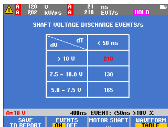
Motor shaft voltage discharge event counts
