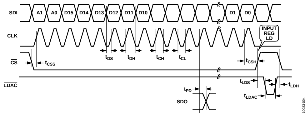
Figure 2. Timing Diagram
