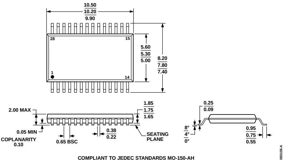
COMPLIANT TO JEDEC STANDARDS MO-150-AH Figure 4. 28-Lead Shrink Small Outline Package [SSOP] (RS-28) Dimensions shown in millimeters
