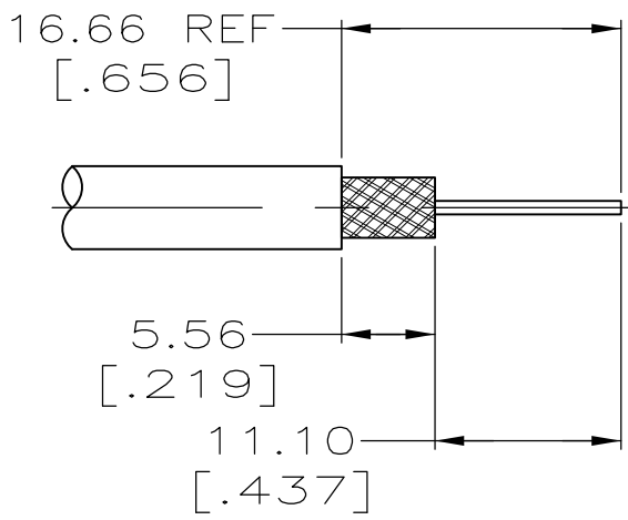
RECOMMENDED STRIP LENGTH SCALE 2:1
