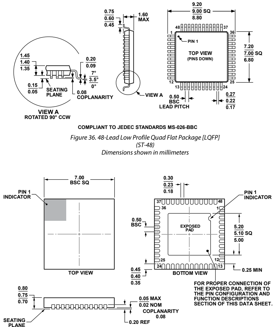
COMPLIANT TO JEDEC STANDARDS MO-220-WKKD. Figure 37. 48-Lead Lead Frame Chip Scale Package [LFCSP] 7 mm × 7 mm Body and 0.75 mm Package Height (CP-48-4) Dimensions shown in millimeters
