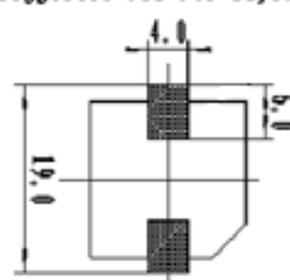
Suggested Pad PCB-Layout
