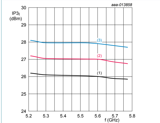
T_{amb} = 25\text{ }^{\circ}\text{C} ; V_{I(CTRL)} = 0\text{ V} ; two tone; 5 MHz spacing; P_i = -5\text{ dBm} ; bypass mode V_{CC} = V_{I(CTRL)} = 3.0\text{ V} V_{CC} = V_{I(CTRL)} = 3.3\text{ V} V_{CC} = V_{I(CTRL)} = 3.6\text{ V}
