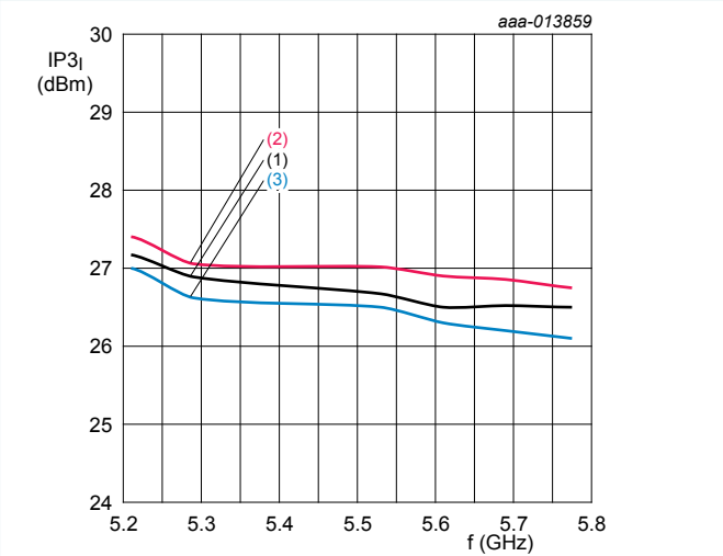
V_{CC} = 3.3\text{ V} ; V_{I(CTRL)} = 0\text{ V} ; two tone; 5 MHz spacing; P_i = -5\text{ dBm} ; bypass mode T_{amb} = -40\text{ }^{\circ}\text{C} T_{amb} = +25\text{ }^{\circ}\text{C} T_{amb} = +85\text{ }^{\circ}\text{C}
