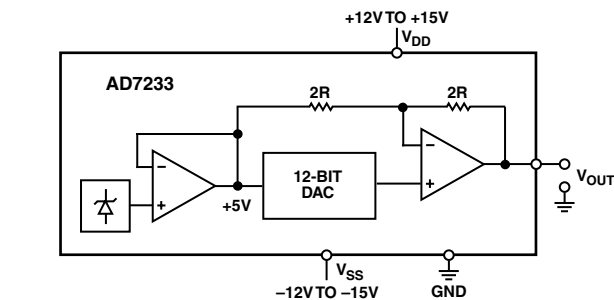
Figure 4. Circuit Configuration
