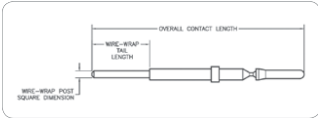
Wire-Wrap Contact
