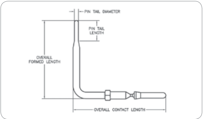
PC Right Angle Contact
