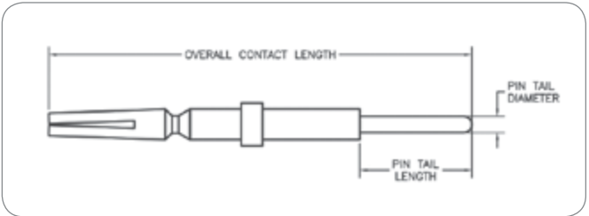
PC Tail Contact
