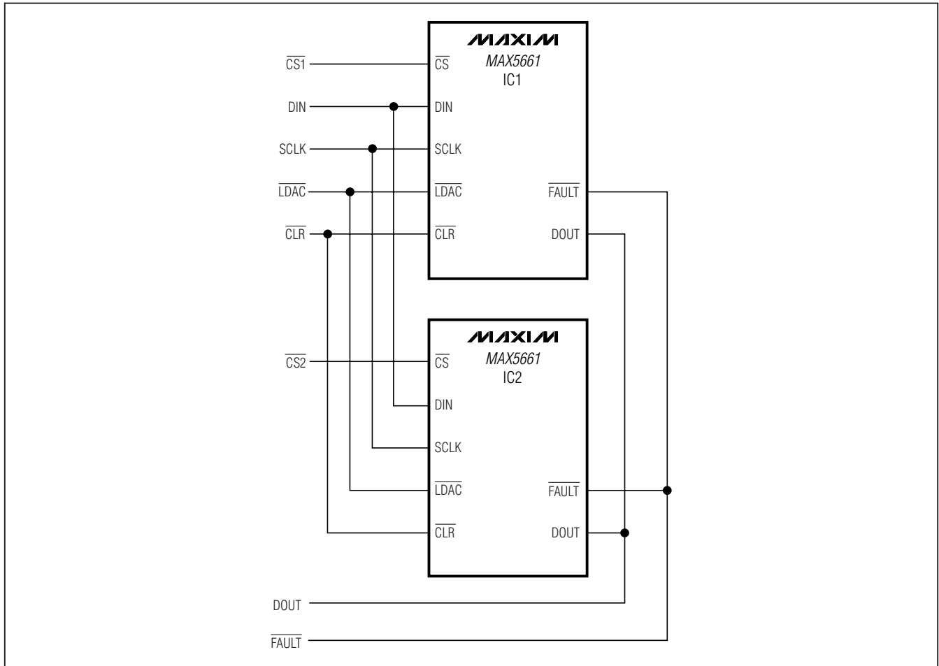
Figure 10. Address Two MAX5661 Devices Through Separate \overline{\text{CS}} Lines
