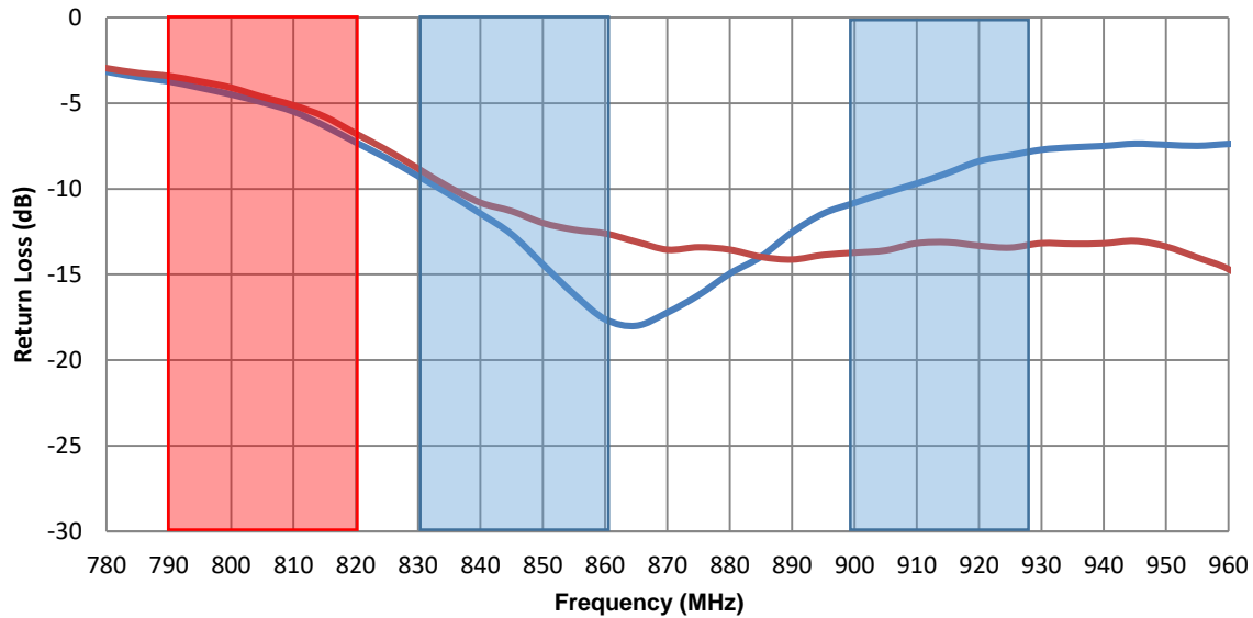
Return Loss
