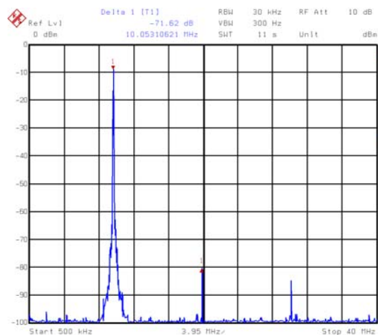
FIGURE 8. ONE TONE AT 10.1MHz, 80MSPS CLOCK (71dBc - NYQUIST, 6dB PAD)
