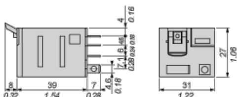
\frac{10000}{1000000} = 0.01
