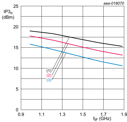
Measured from A_RF IN to IFOUT1. Low band; single activated IF path; V CC = 5 V; T amb = 25 °C; tone separation = 33 MHz. (1) High gain mode (2) Medium gain mode (3) Low gain mode
