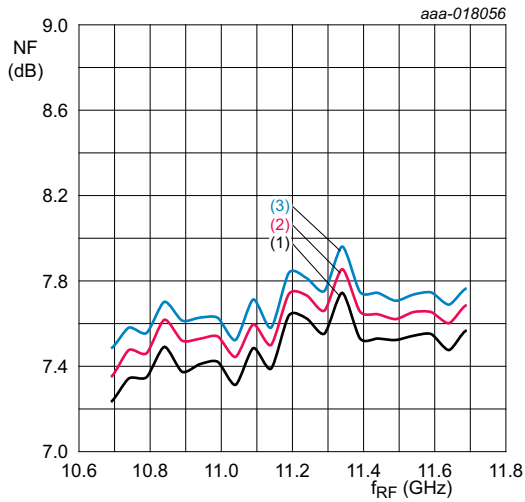
Measured from B_RF IN to IFOUT1. Low band; V_{CC} = 5\text{ V} ; T_{amb} = 25\text{ }^{\circ}\text{C} . (1) High gain mode (2) Medium gain mode (3) Low gain mode
