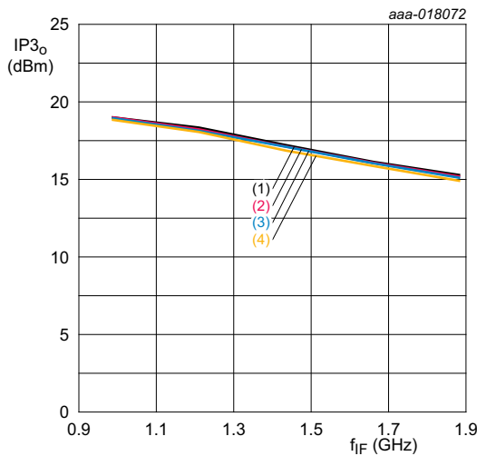
Measured from A_RF IN to IFOUT1. Low band; high gain mode; V CC = 5 V; T amb = 25 °C; tone separation = 33 MHz. (1) 1 activated IF path (2) 2 activated IF paths (3) 3 activated IF paths (4) 4 activated IF paths
