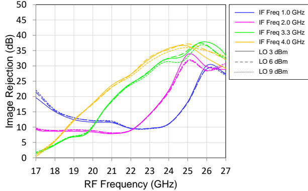
LSB Image Rejection vs. RF vs. IF and LO Power State: Min Gain
