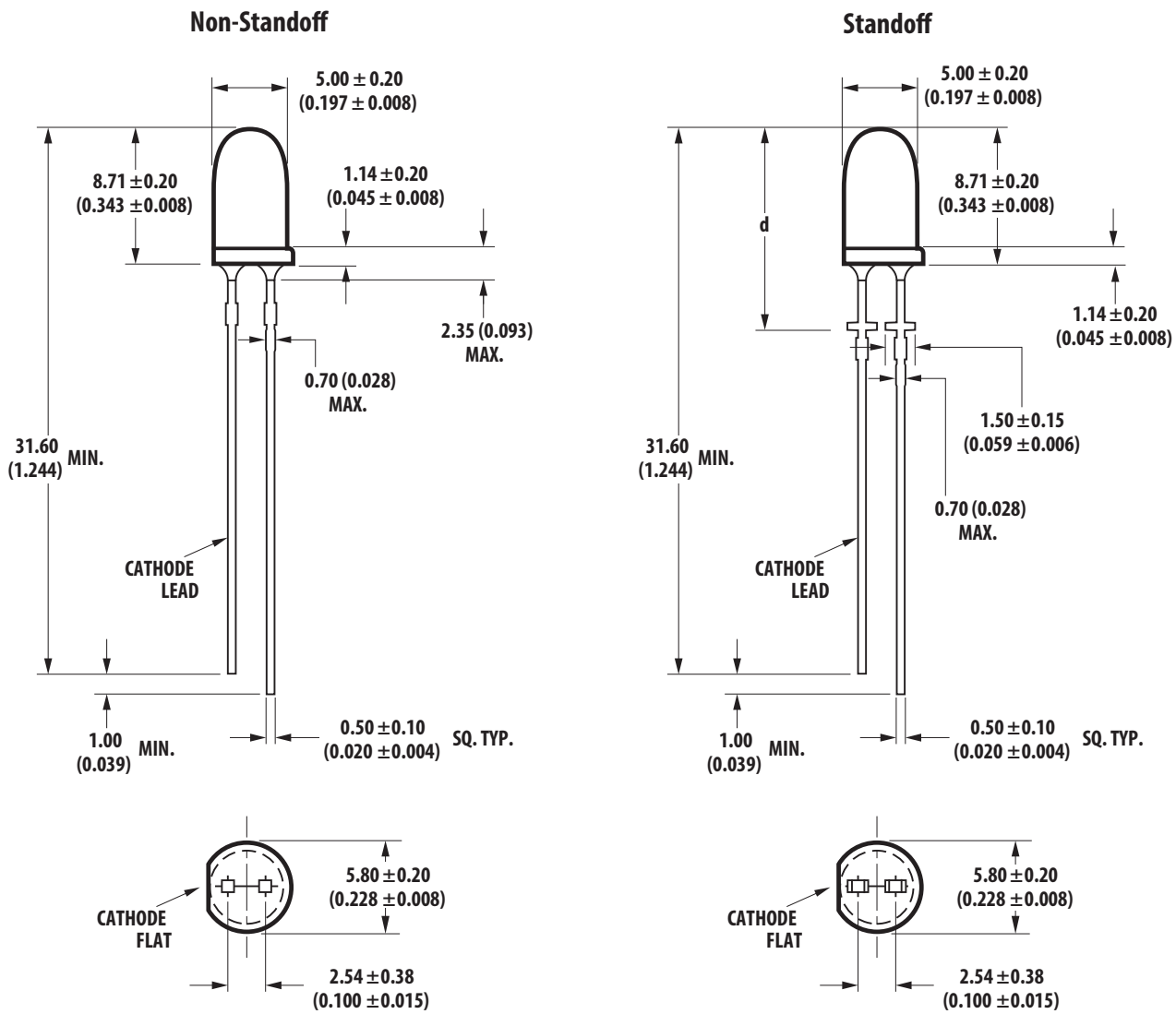
Figure 1: Package Dimensions
