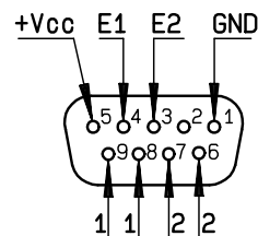
D-Sub connector
