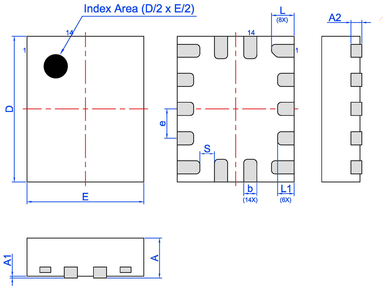
14 Lead STQFN Package
