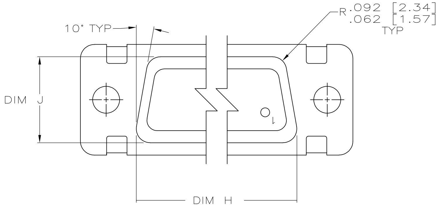
VIEW Z-Z
