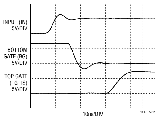
LTC4442 Driving 3000pF Capacitive Loads
