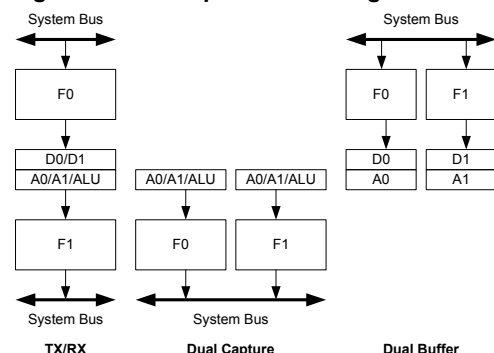
Figure 7-9. Example FIFO Configurations
