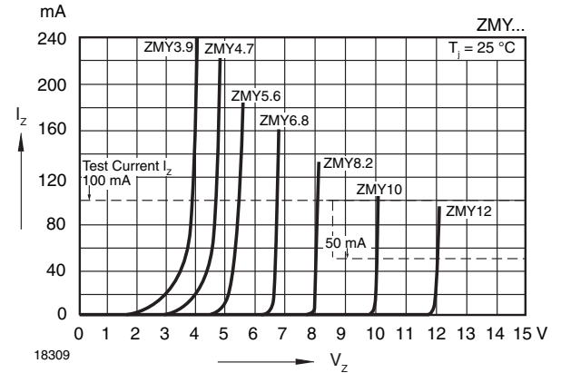
Fig. 6 - Breakdown Characteristics
