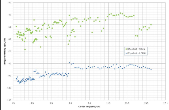
Figure 16. 10 kHz and 2.5 MHz fractional spur (integer boundary, 5.0 V supply, F_{PFD}=50 MHz)
