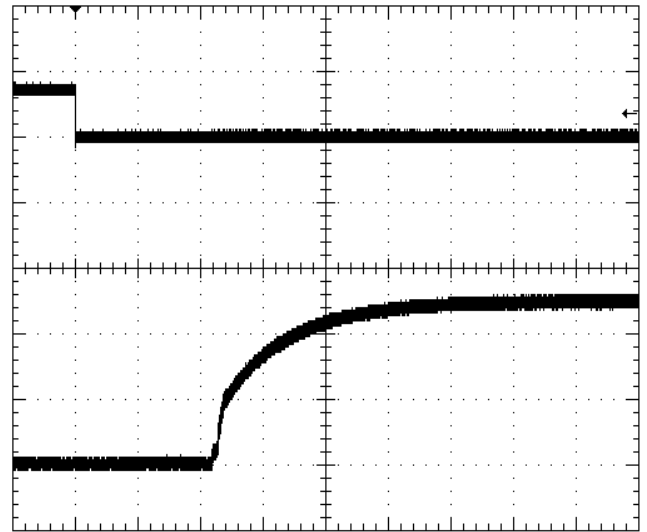
Fig-5: Turn-on transient at full rated load current (resistive) plus 20,000 \mu F at Vin=48V, triggered via ON/OFF pin. Top trace: ON/OFF signal (5V/div). Bottom trace: output voltage (2V/div). Time scale: 10ms/div
