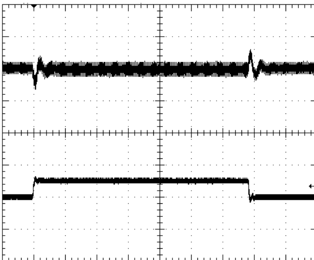
Fig-6: Output voltage response to load current step-change (20A-30A-20A) at Vin=48V. Top trace: Output voltage (200mV/div). Bottom trace: load current (20A/div). Current slew rate: 5A/ \mu s. Co=470 \mu F Low Z EL-con + 10 \mu F ceramic. Time scale: 200 \mu s/div
