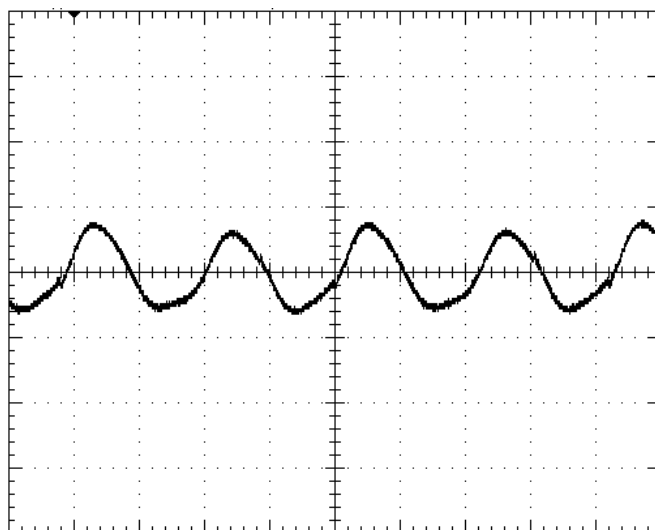
Fig-10: Input reflected ripple current, I_c (500mA/div), measured through 10μH at the source at full rated load current and V_{in}=48V . Time scale: 1μs/div.
