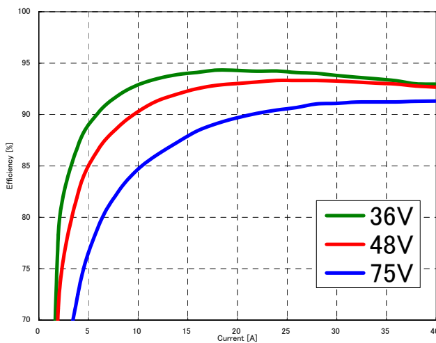
Fig-2: Efficiency vs. load current and input voltage for converter mounted horizontally with airflow from pin 3 to pin 1 at a rate of 400LFM (2.0m/s) and T_a=25^{\circ}C .
