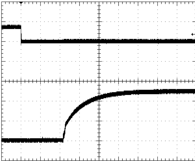
Fig-4: Turn-on transient at full rated load current (resistive) with 10 \mu F tantalum + 1 \mu F ceramic capacitor at Vin=48V, triggered via ON/OFF pin. Top trace: ON/OFF signal (5V/div). Bottom trace: output voltage (2V/div). Time scale: 2ms/div
