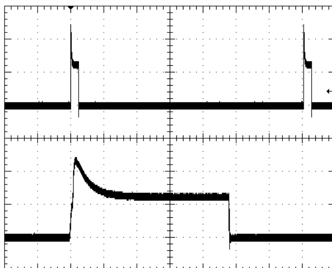
Fig-12: Load current (top trace, 50A/div, 40ms/div) into a 10mΩ short circuit during restart, at V_{in} = 48V . Bottom trace (50A/div, 2ms/div) is an expansion of the top trace.
