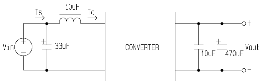
Fig-8: Test Set-up for measuring input reflected ripple current.
