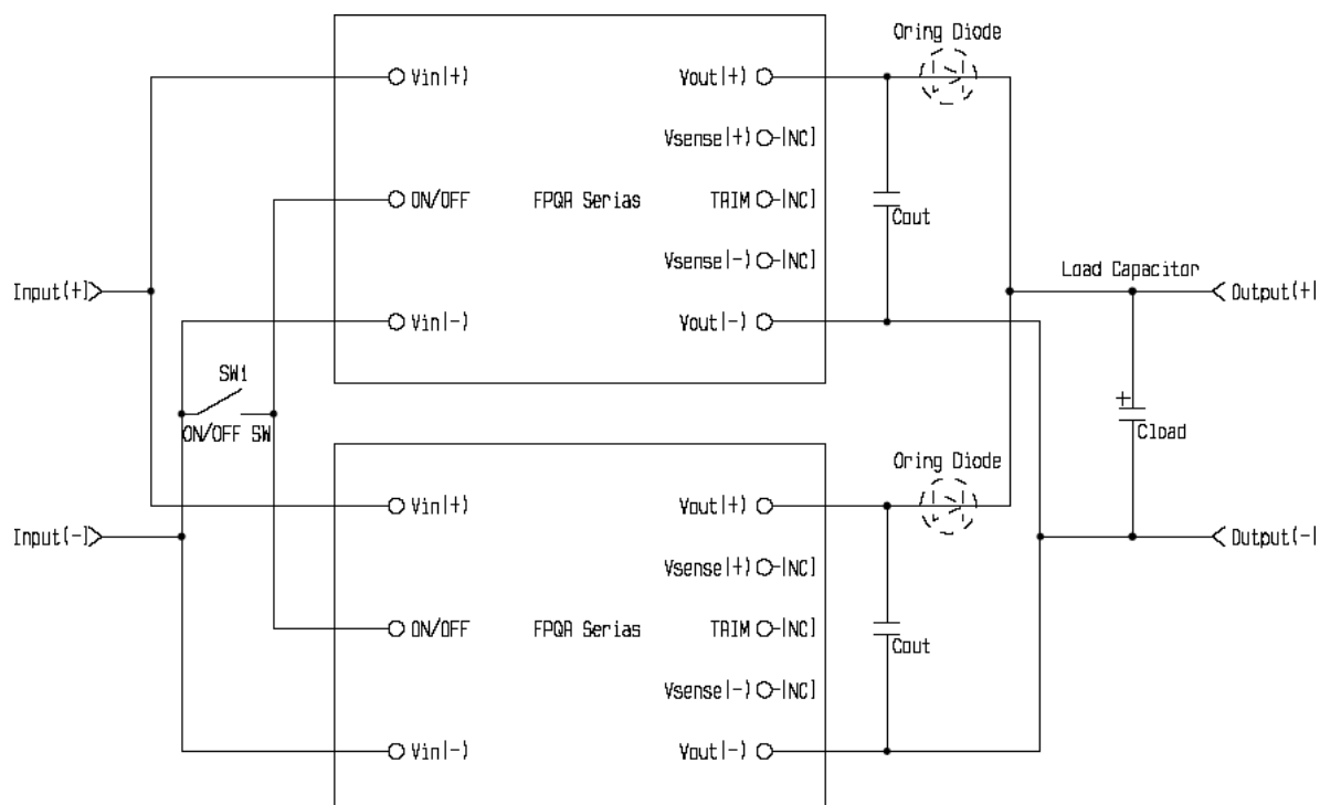
Sch-1 : Circuit for using the parallel option
