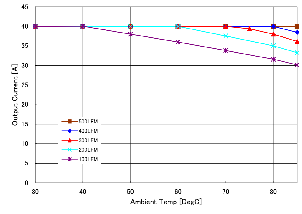
Fig-1: Available load current vs. ambient temperature and airflow rates for V_{in}=48V . Maximum component temperature \leq 125^{\circ}C
