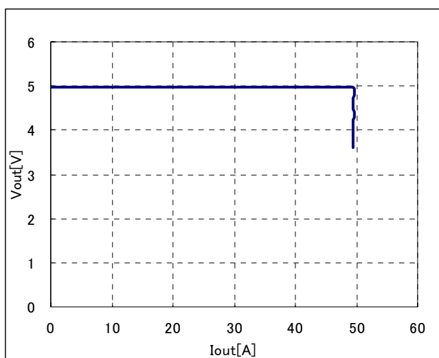
Fig-11: Output voltage vs. load current showing current limit point and converter shutdown point. ( V_{in} = 48V )
