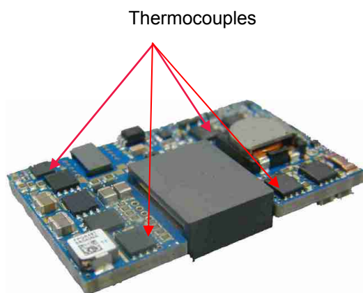
Fig. G: Location of thermocouples for thermal testing
