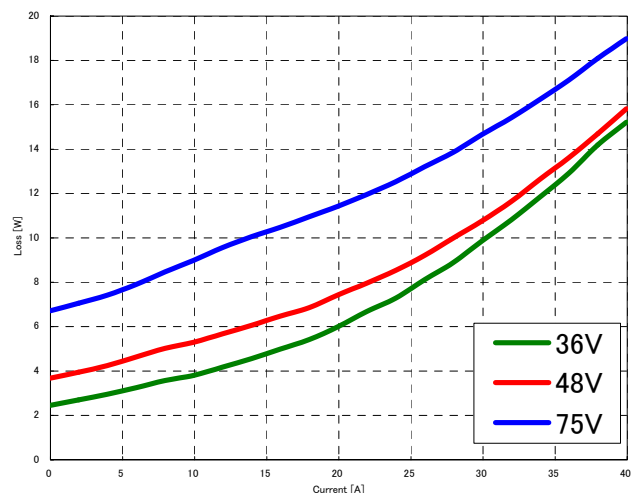
Fig-3: Power dissipation vs. load current and input voltage for converter mounted horizontally with airflow from pin 3 to pin 1 at a rate of 400LFM (2.0m/s) and T_a=25^{\circ}C .
