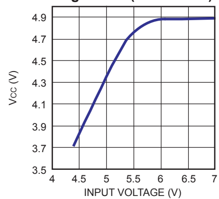
Vcc Regulator Line Regulation ( I_{CC} = 10mA )
