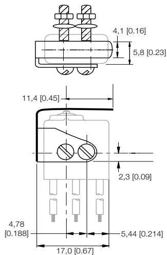
Figure 11. JM-1 Dimensions
