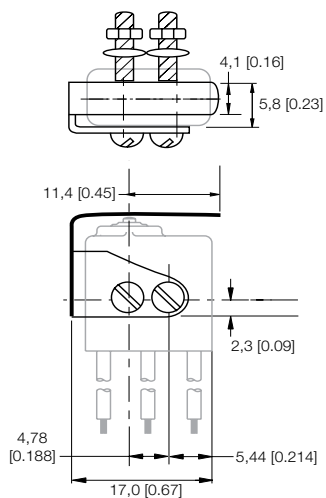
Figure 11. JM-1 Dimensions
