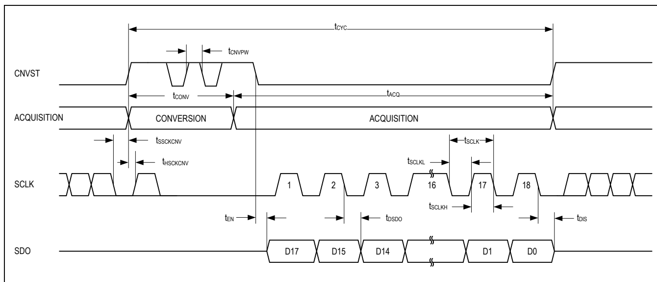
Figure 6. \overline{\text{CS}} Mode 3-Wire, No-Busy Indicator Serial Interface Timing (SDI High)
