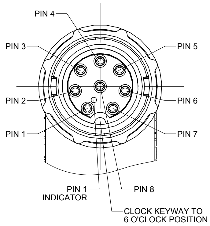
PIN CALLOUT VIEW FROM MATING SIDE OF CONNECTOR SCALE=3:1
