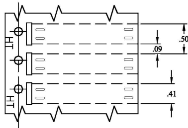
Figure 1 CM-SCE-1/4 INCH
