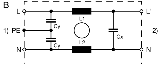
EMI filtering of equipment emissions
