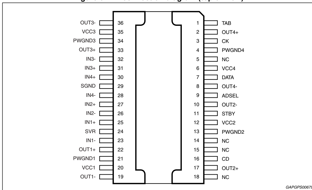
Figure 3. Pin connection diagram (top of view)
