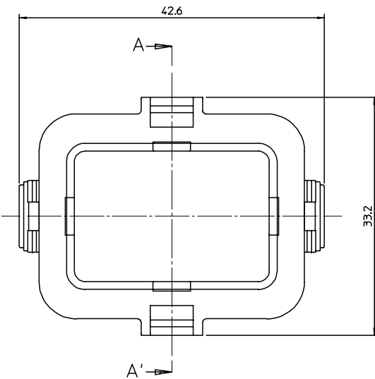
VIEW "A"
