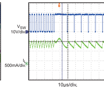
Short Protection
