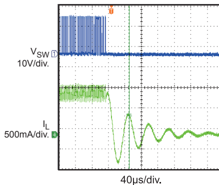
Open Protection
