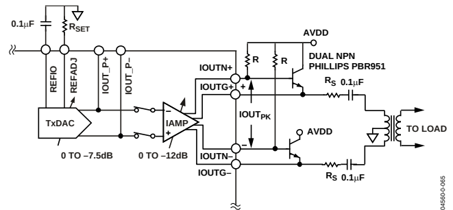
Figure 65. Voltage-Mode Operation
