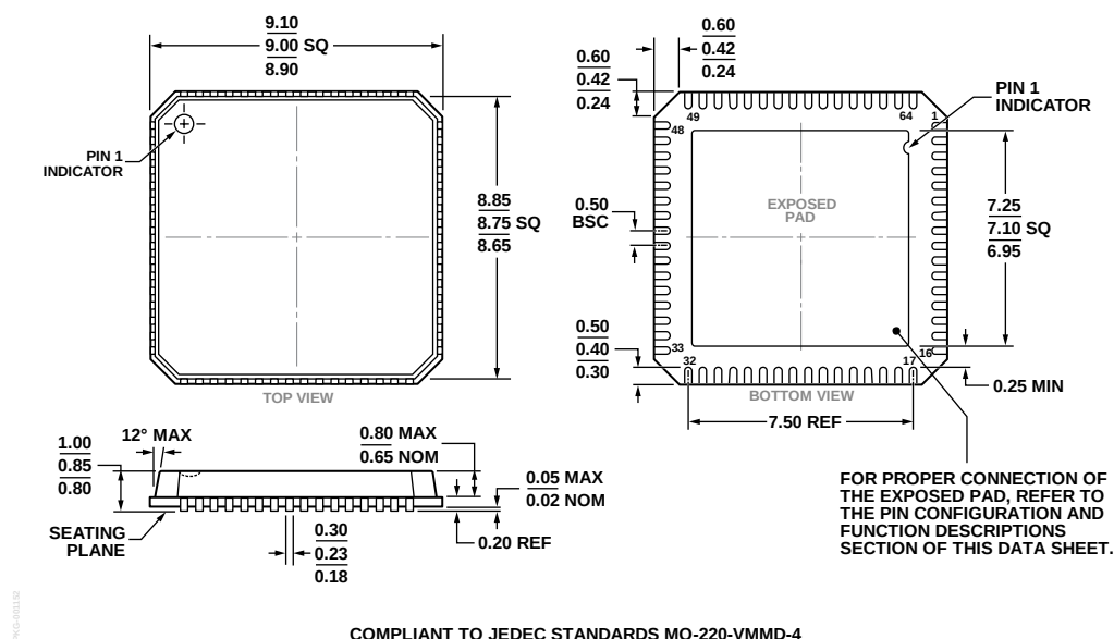
Figure 85. 64-Lead Lead Frame Chip Scale Package [LFCSP_VQ] 9 mm × 9 mm Body, Very Thin Quad (CP-64-3) Dimensions shown in millimeters
