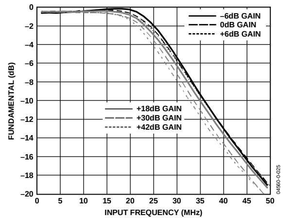
Figure 25. Rx Low-Pass Filter Amplitude Response vs. RxPGA Gain (LPF's f_{-3\text{ dB}} = 33 MHz)
