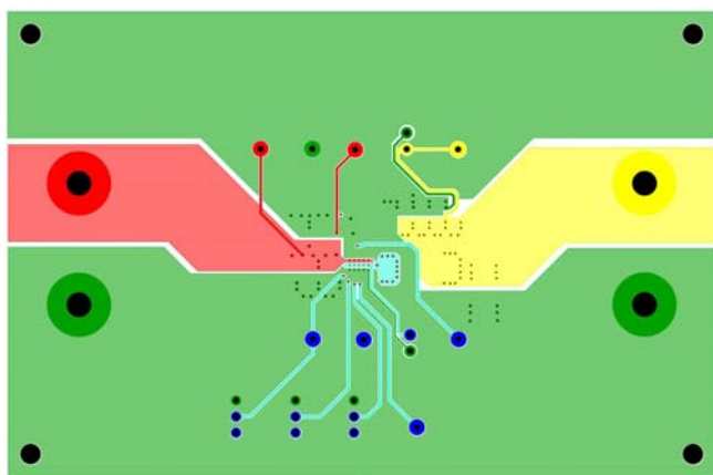
FIGURE 6. LAYER 3
