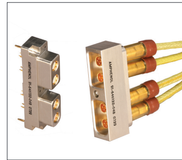
Compliant Pin Quadrax Board Level Connector
