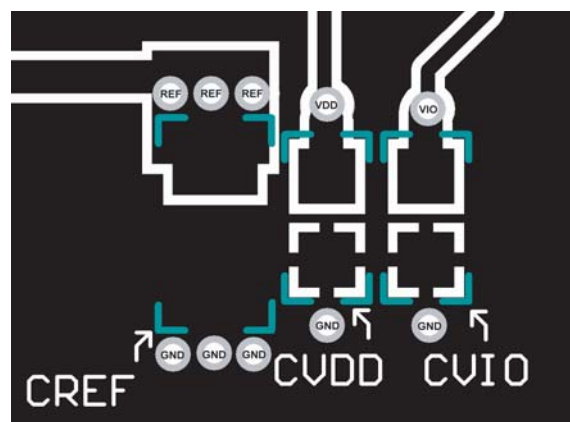
Figure 66. Example Layout of the AD4002 (Bottom Layer)
