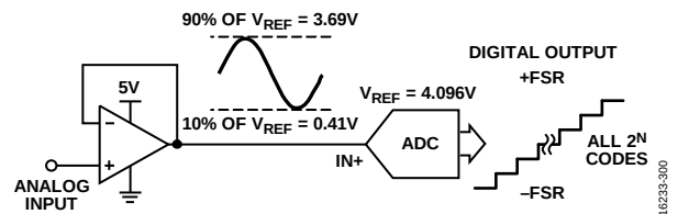
Figure 40. Span Compression
