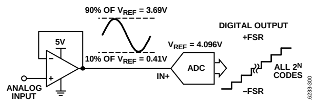
Figure 40. Span Compression
