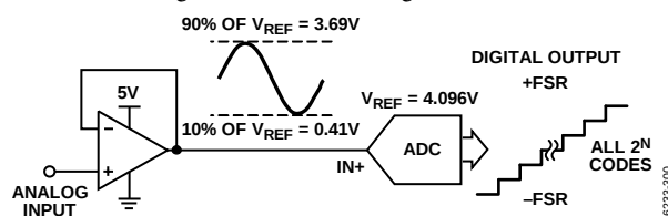
Figure 40. Span Compression
