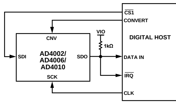
Figure 57. \overline{\text{CS}} Mode, 4-Wire Turbo Mode Connection Diagram
